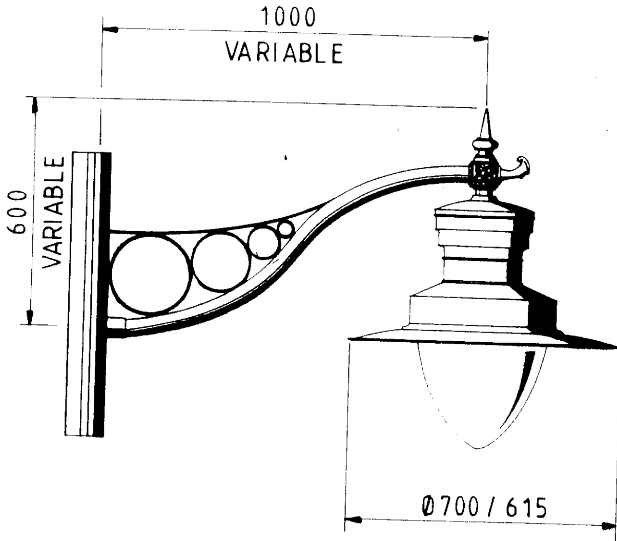
PRESTON ON CATHRINGTON 2 COLUMN MOUNTING
