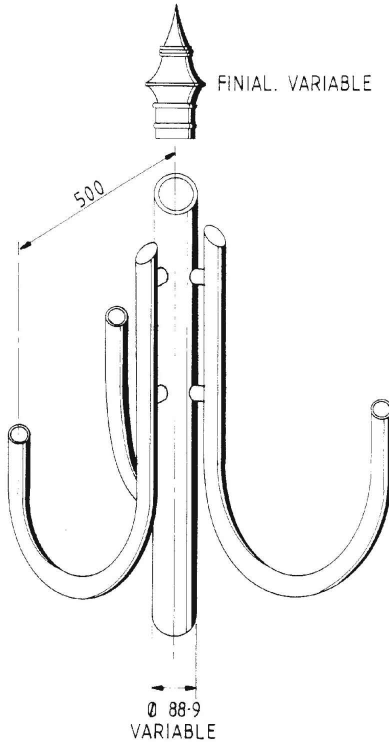
PLAIN 'U' ARM BRACKET X 3 CAN BE INVERTED
