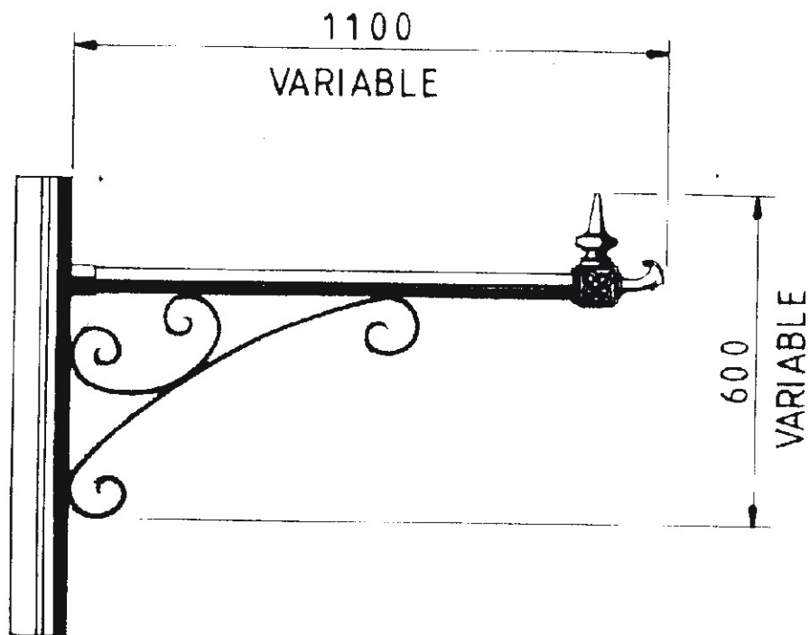
BANBURY COLUMN MOUNTING
