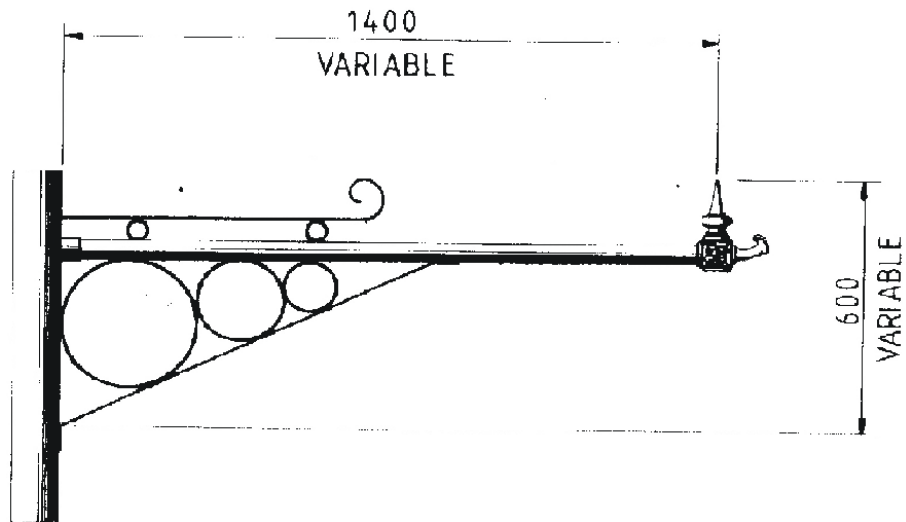
EDINBURGH SPECIAL COLUMN MOUNTING
